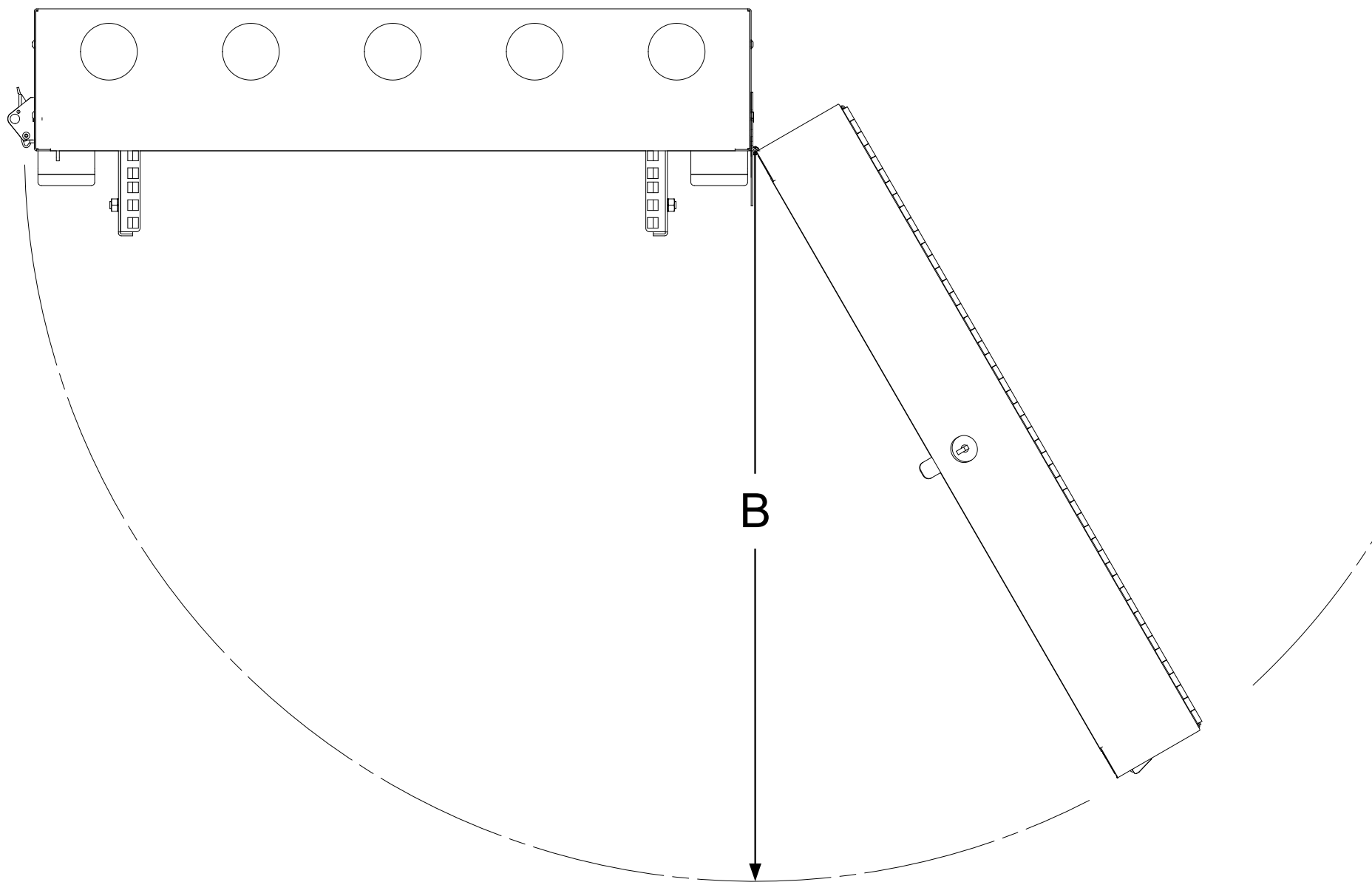
FRONT COVER SWING IS REVERSIBLE TOP VIEW
